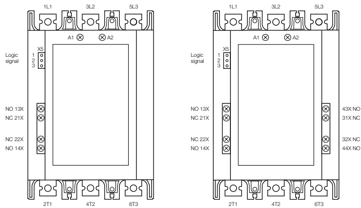
AF400 ... AF1250-30-11
