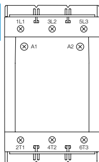
AF116 ... AF370-30-00
