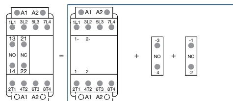
Combination 11 = AF09 ... AF38..-40-00 + CA4-10 + CA4-01
