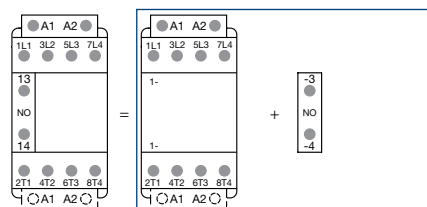
Combination 10 = AF09 ... AF38..-40-00 + CA4-10
