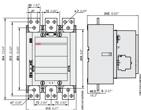
AF1250
