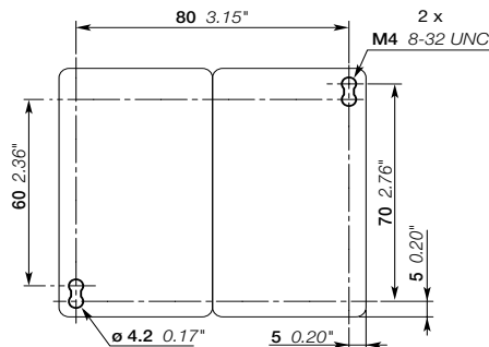
AF09N00R, AF12N00R
