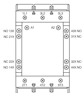
AF116 ... AF370-30-22
