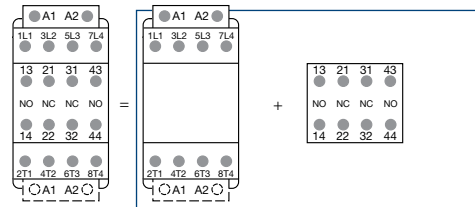
Combination 22 = AF09 ... AF38..-40-00 + CA4-22E
