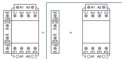
Combination 11 = CAL4-11 + AF09 ... AF38..-40-00
