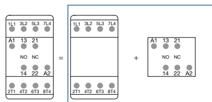
Combination 11 = AF09 ... AF38..-40-00 + CAT4-11E
